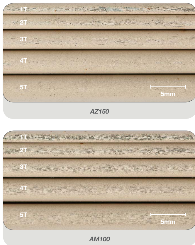
Figure 8: Prepainted bend samples exposed in an unwashed marine environment for 51 months.
