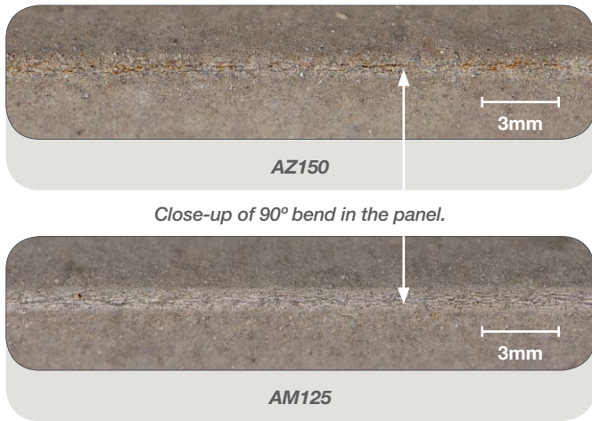
Figure 5: Close-up photographs of the 90° bend of unpainted samples exposed in a marine environment after 18 months (washed).
