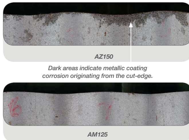
Figure 2: Unpainted sheltered walling (i.e. unwashed) in a severe marine environment after 50 months.
