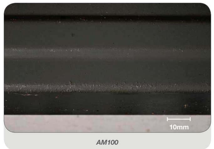
Figure 6: Unpainted samples of AZ and AM with various bend diameters, exposed in a sheltered (i.e. unwashed) severe marine environment for 45 months.
