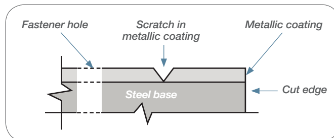
Figure 1: Schematic of a cut edge (not to scale).
