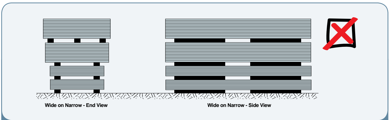
Figure 11c: Incorrect stack construction
