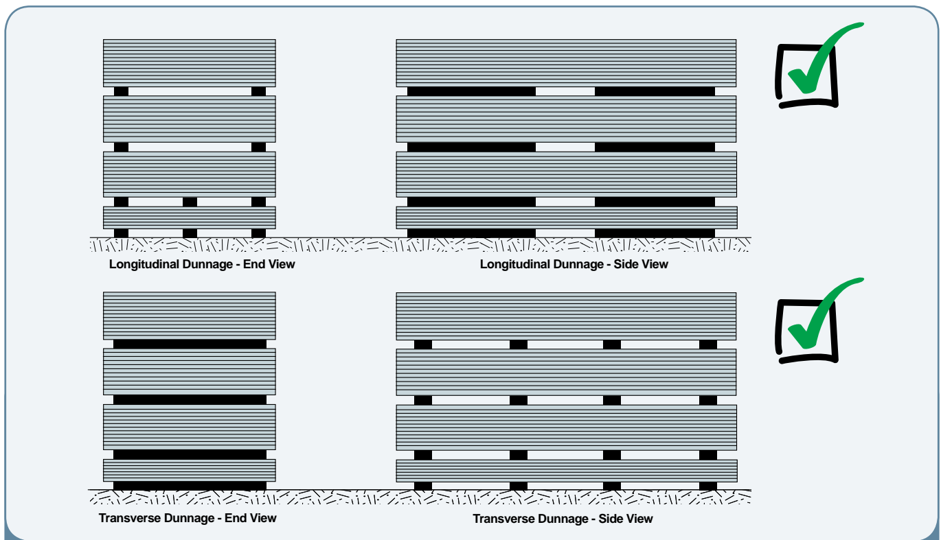
Figure 11a: Correct dunnage placement
