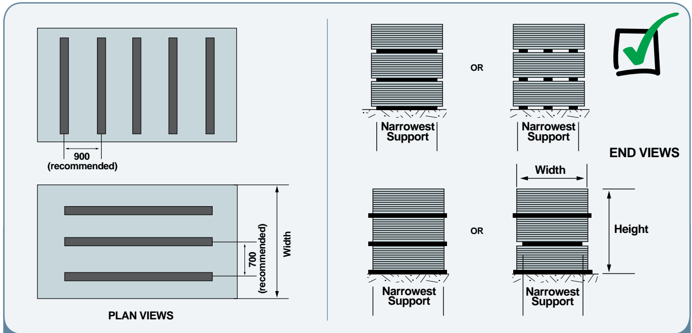
Figure 10: Dunnage placement and stack height
