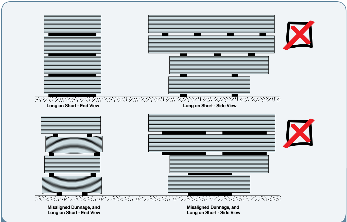
Figure 11b: Incorrect stacking and dunnage placement
